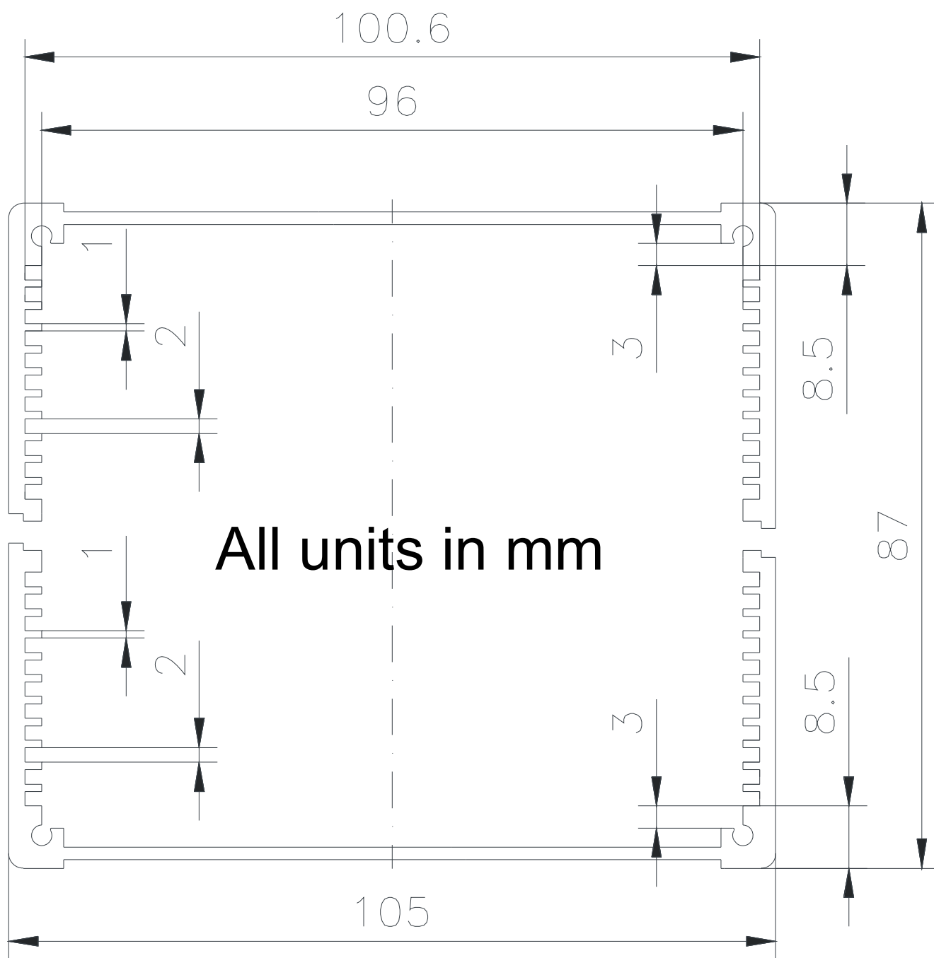
Microstar Laboratories SBE slot positions
